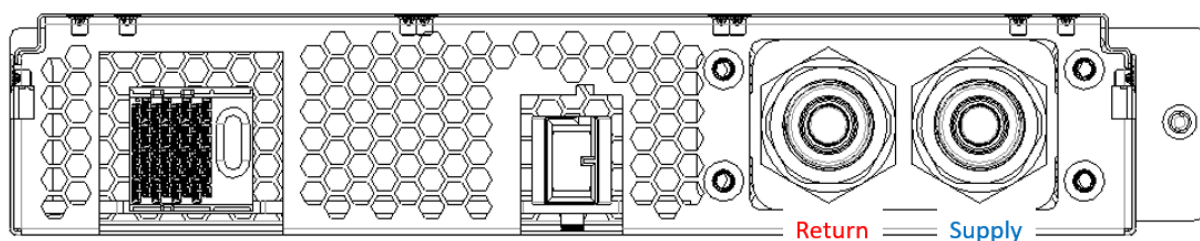
Figure 56. Brick side supply and return
