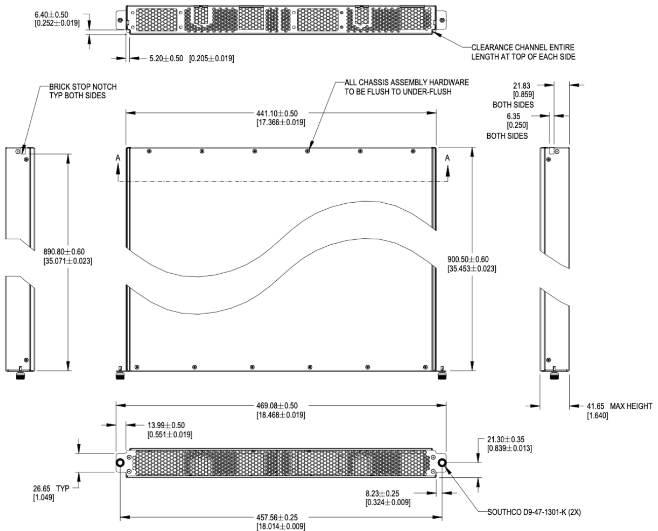
Figure 77. Brick dimensions
