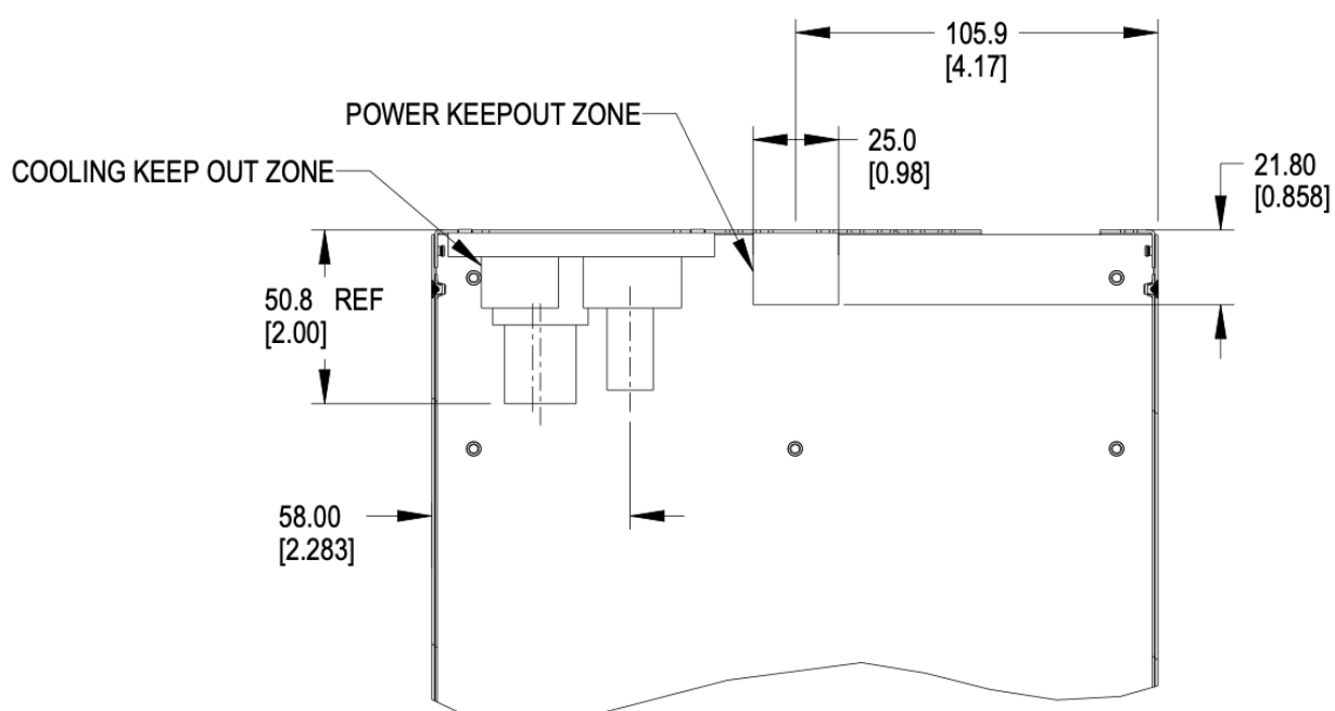
TOP SECTION KEEPOUT ZONE DETAILS
