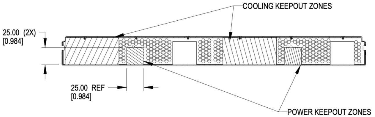
Figure 112. Brick keep-out zone
